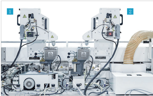
Gluing unit and pre-melter: Quick-change application unit with hot melt glue supply from top. On-demand availability and perfect glue quality with Quickmelt. (1 # optional PUR coating)
