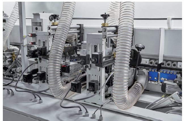
Fine trimming unit: Process overhang edge from top and bottom (rough trimming unit as option).
