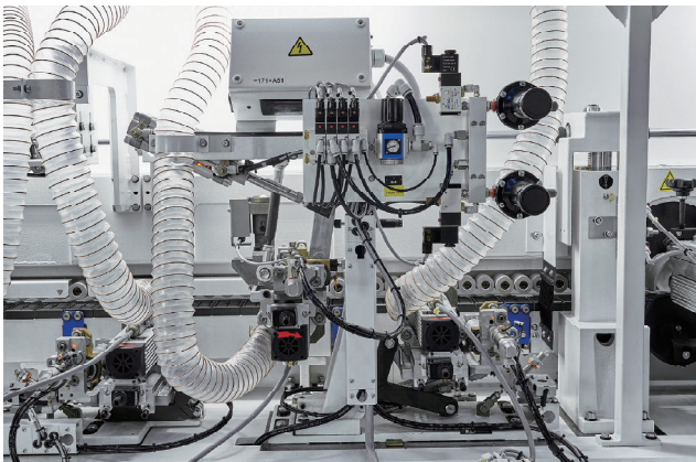
Profile trimming unit: For profile trimming of thick PVC edges. Workpiece thickness up to 60 mm. Standard pneumatic on/off. For easy operating. Max. feed speed 25 m/min.
