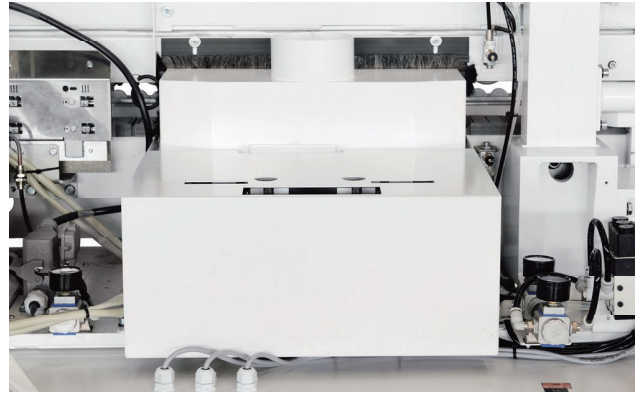
Joint trimming unit: Perfect cut and long service life due to diamond tipped tools for optimum edge joint quality.
