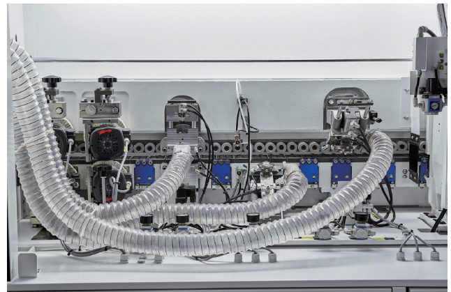
Double polishing device: Meets the coating requirements of two different colors and improves the surface appearance quality. Standard 1 pic polishing device.
